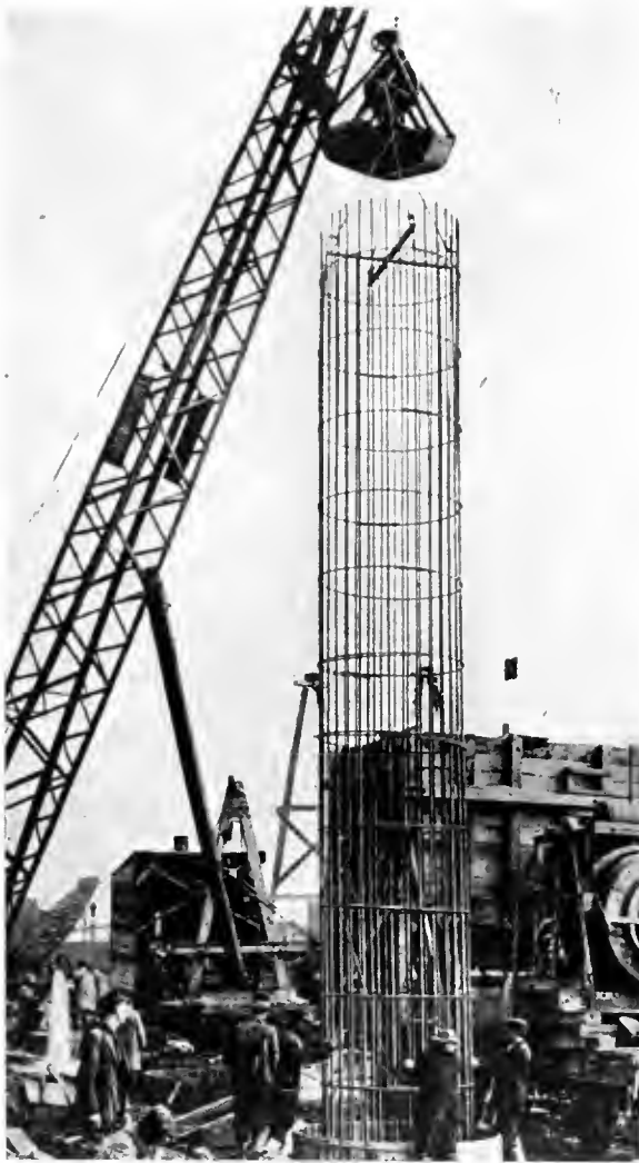
PLACING REINFORCED STEEL CAGE IN CYLINDRICAL WELL
